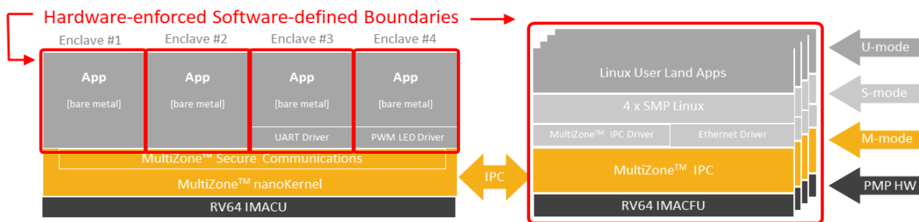
Fig. 2. Multi Zone Enclave For Linux - System Architecture
